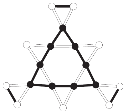
Figure 4. Magnetic exchange pathways between cobalt ions in \text{Co}_3\text{-(SO}_4)_3\text{(OH)}_2\text{[enH}_2\text{]} . Cobalt ions that form a single [\text{Co}_9\text{O}_{36}] triangular cluster are denoted by solid circles. Antiferromagnetic couplings across shared octahedral edges are likely to be the strongest exchange interactions and are indicated by solid bonds while the weaker interactions via common octahedral vertices are represented by open bonds. All nonmetal atoms are omitted for clarity.
